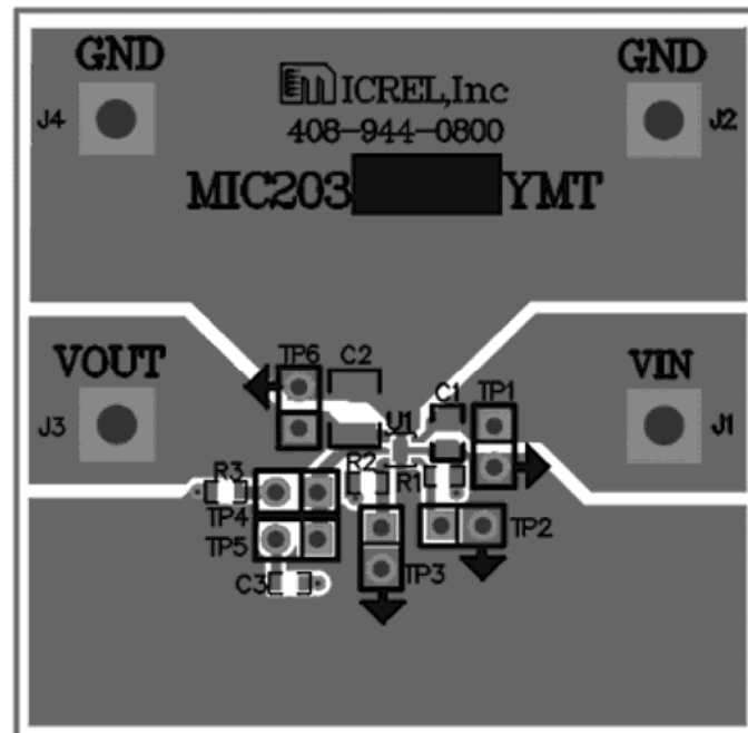
MIC2039xYMT Evaluation Board – Top Layer
